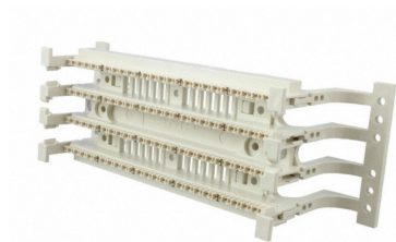
110Connect XC System Cross-Connect Wiring Block with Legs, 100-pair, Category 5e, .110 punch down
